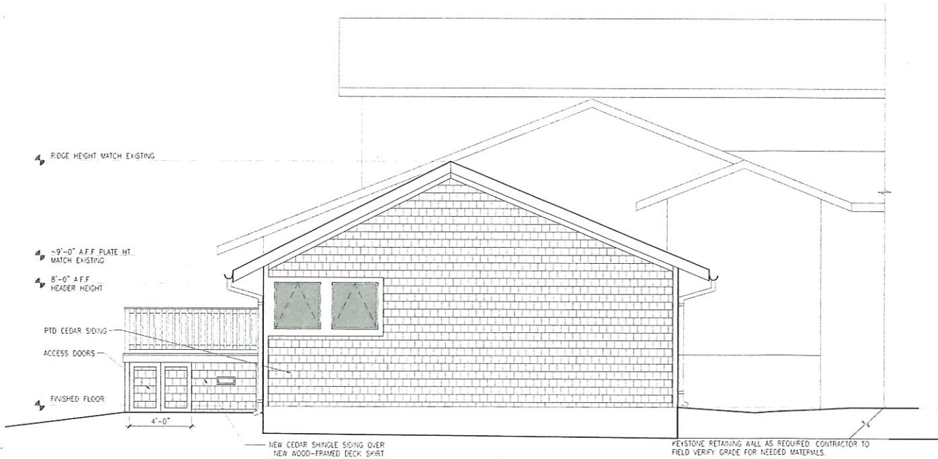
2 EXTERIOR ELEVATIONS SCALE: 1/4" = 1'-0"
