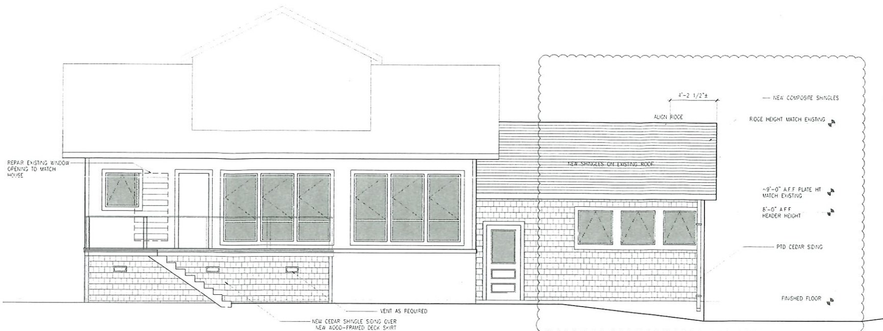
1 EXTERIOR ELEVATIONS SCALE: 1/4" = 1'-0"
