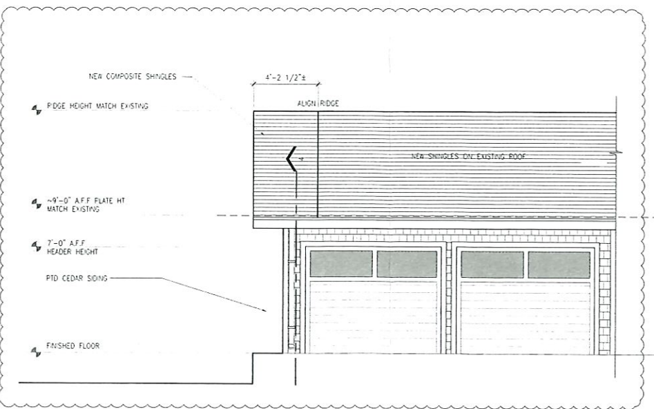
3 EXTERIOR ELEVATIONS SCALE: 1/4" = 1'-0"
