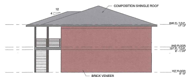
NORTH ELEVATION
