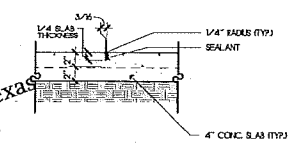
4 SAW CUT JOINT SCALE 1/2" = 1'-0"
