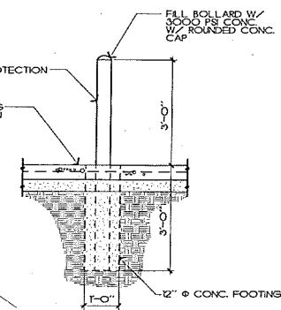
3 PROTECTION BOLLARD SCALE 1/2" = 1'-0"
